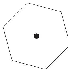
Figure 3. Regular hexagon with rotational symmetry of order 6.
